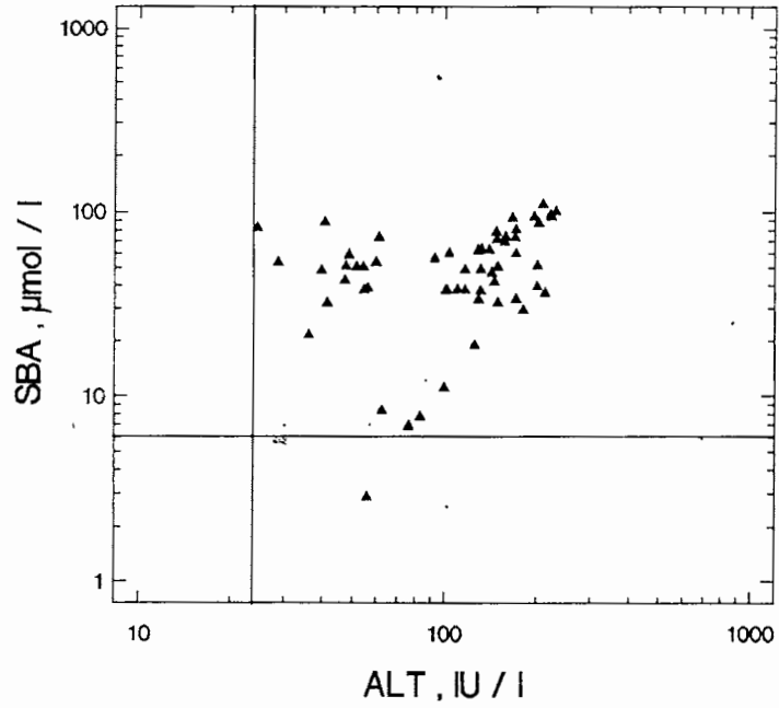
FIG. 3. Relationship between (SBA \mu\text{mol}/\text{L} ) and (ALT IU/L) in obstructive jaundice. The vertical and horizontal lines within the X and Y axes represents the reference range for SBA and ALT.
