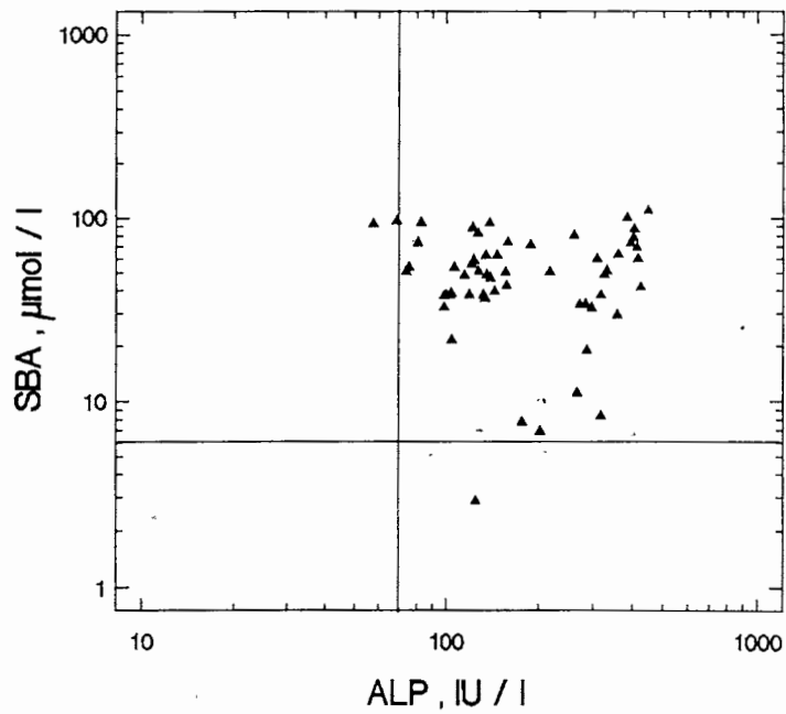
FIG. 4. Relationship between (SBA \mu\text{mol}/\text{L} and alkaline phosphatase (ALP IU/L) in obstructive jaundice. The vertical and horizontal lines within the X and Y axes represents the reference range for SBA and total ALP.
